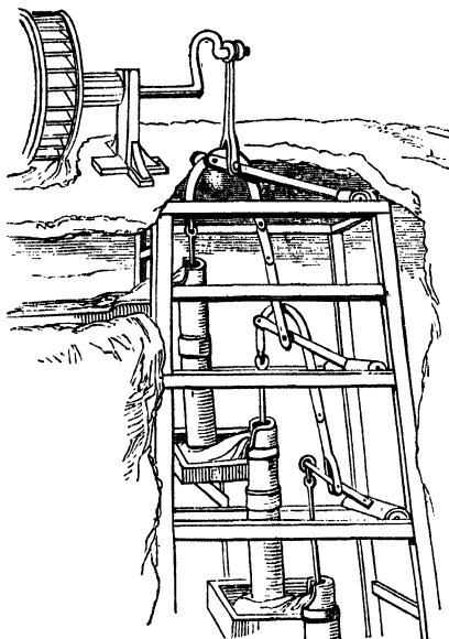
Fig. 200. Pumping Apparatus used three hundred years ago. (Agricola, 1550.)
